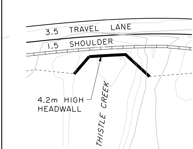
OPTIONAL CULVERT HEADWALL PLAN
