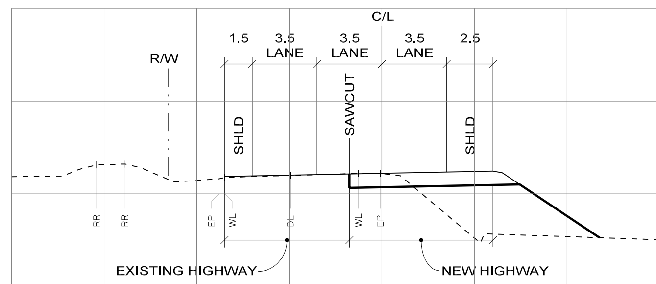
TYPICAL SECTION
