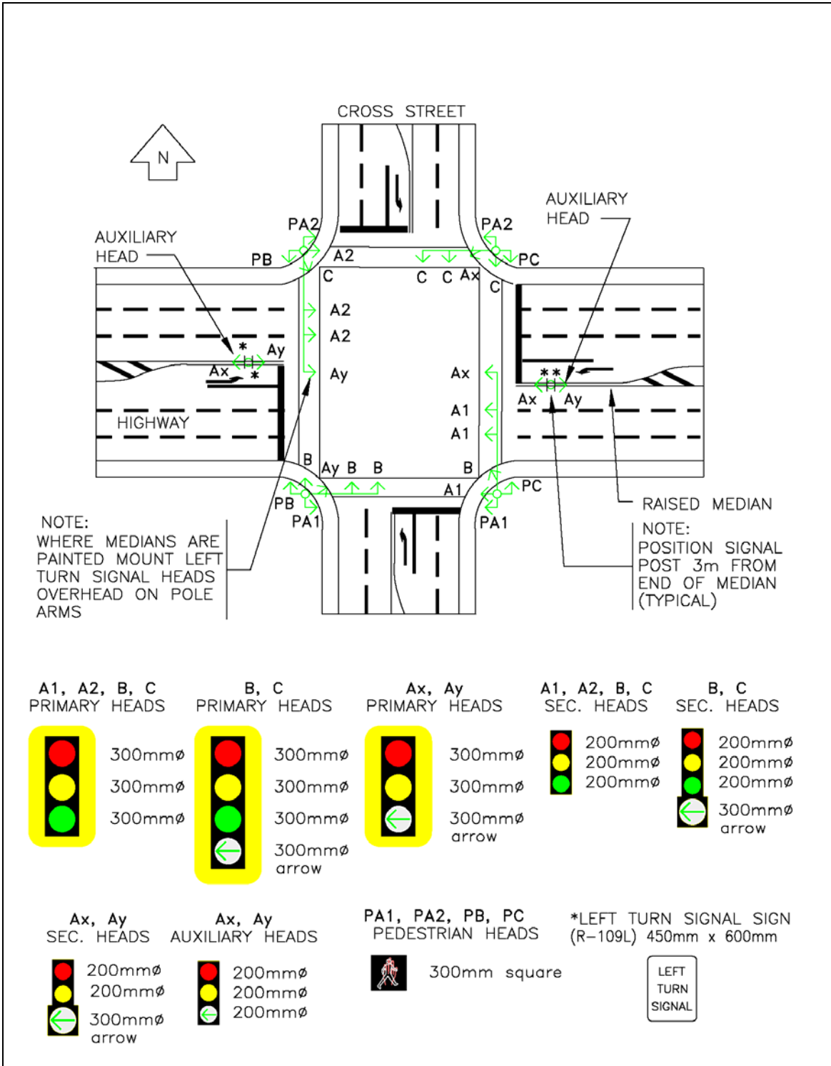
Figure 36. Full intersection with NEMA Dual Ring operation and protected left turn signals (single lane) on highway and split phasing on the cross street
