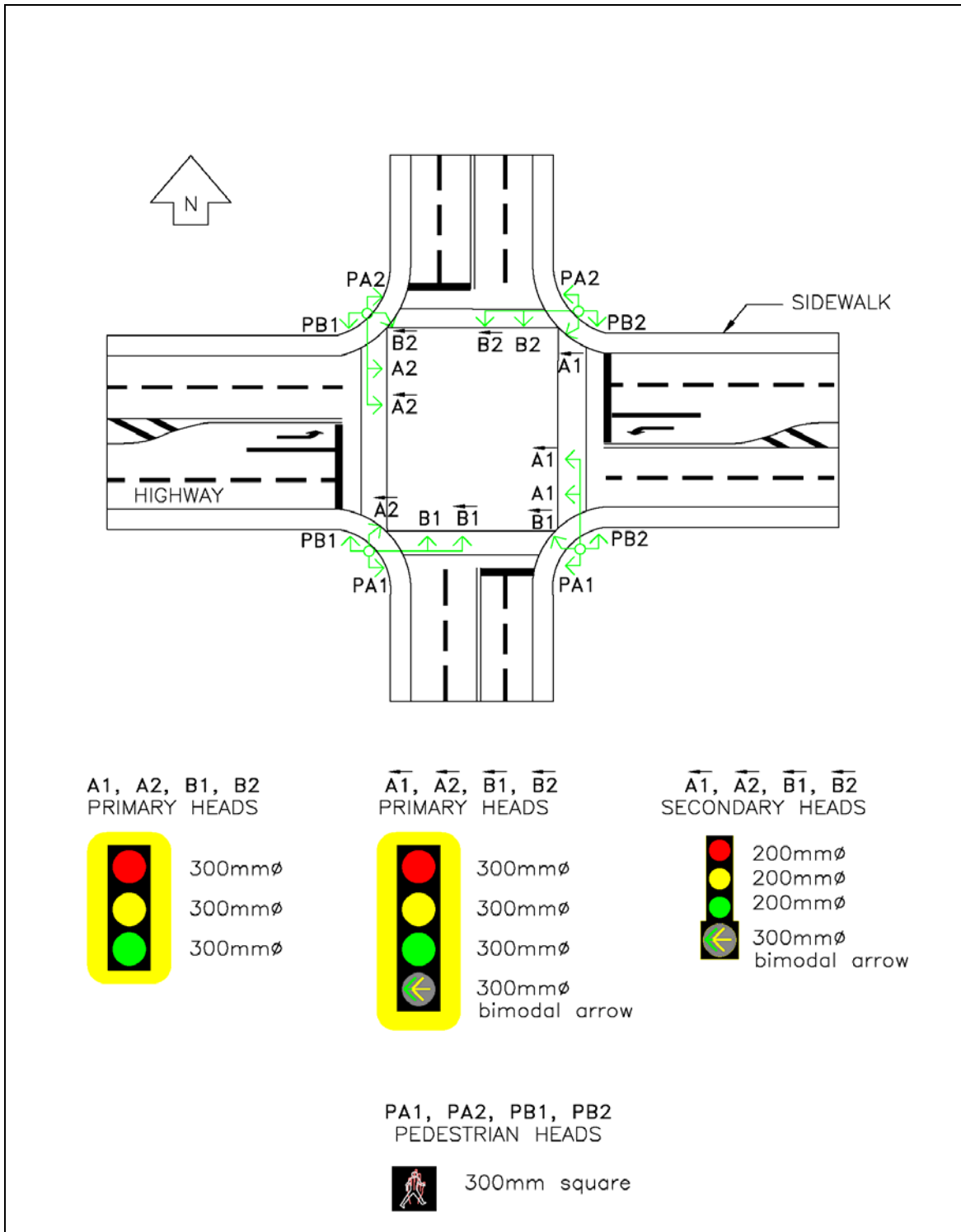
Figure 35. Full intersection with NEMA Dual Ring operation and protected/permissive left turn signals
