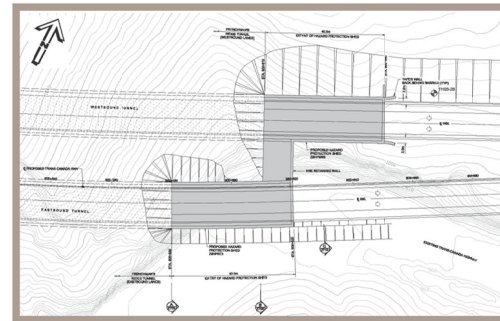
Hazard protection sheds will protect against snow avalanche and rock fall hazards.
